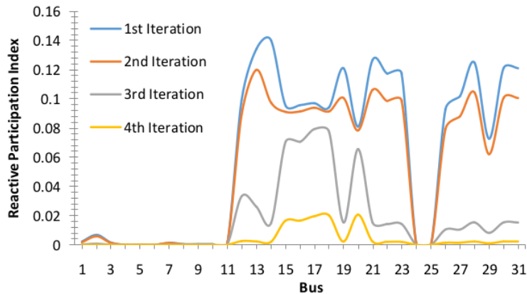
Figure 4. Reactive Participation Index of each load buses
