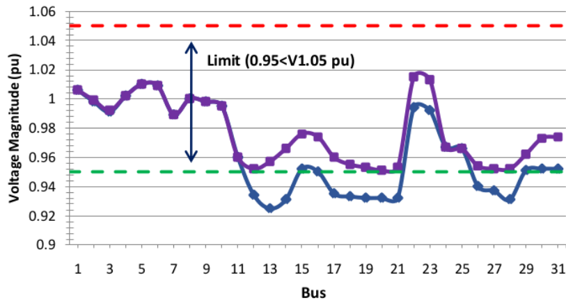
Figure 5. Voltage profile shows an improvement after capacitor installation
