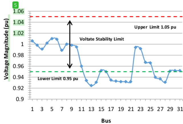
Figure 3. Voltage profile of Selsel system at peakload [23]
